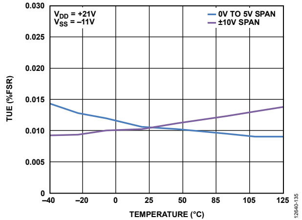
Figure 34. TUE vs. Temperature
