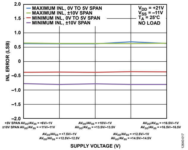
Figure 16. INL Error vs. Supply Voltage
