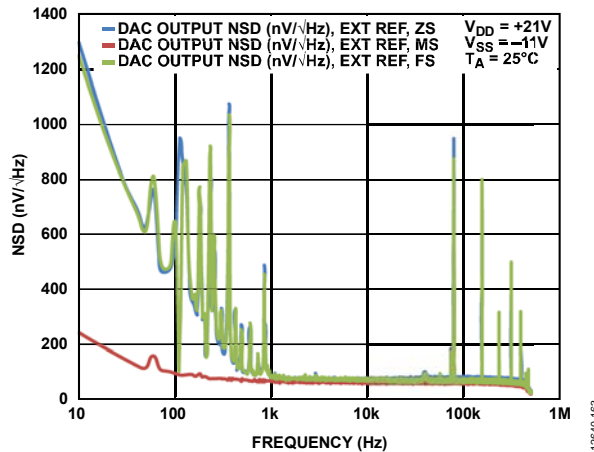
Figure 59. DAC Output Noise Spectral Density vs. Frequency, \pm 10 V Range
