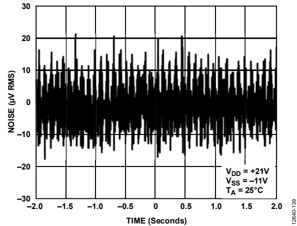
Figure 58. Peak-to-Peak Noise (Voltage Output Noise), 100 kHz Bandwidth
