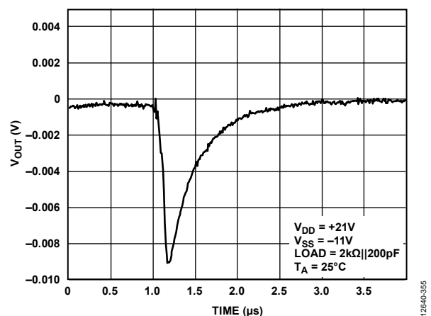
Figure 47. Digital-to-Analog Glitch Energy, ±10 V Range
