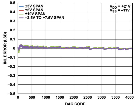
Figure 9. AD5721 INL Error vs. DAC Code, Bipolar Output
