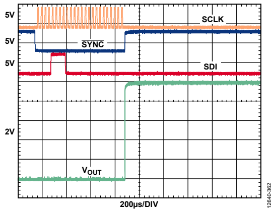
Figure 54. Software Full Reset Glitch from Zero Scale with Output Loaded, \pm 10 V Range
