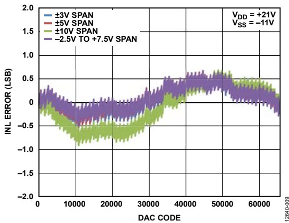
Figure 8. AD5761 INL Error vs. DAC Code, Bipolar Output
