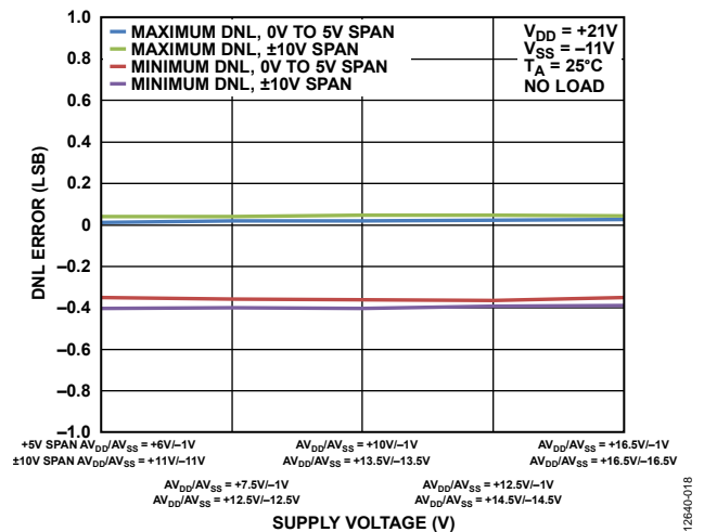
Figure 17. DNL Error vs. Supply Voltage
