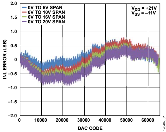
Figure 6. AD5761 INL Error vs. DAC Code, Unipolar Output
