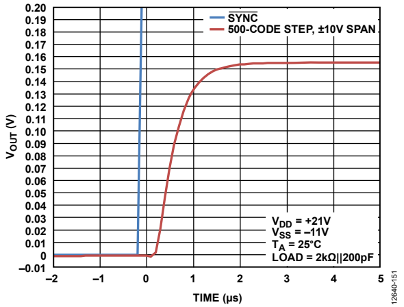
Figure 43. 500-Code Step Settling Time, ±10 V Range
