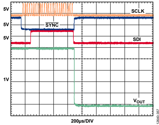
Figure 49. Software Full Reset Glitch from Full Scale with Output Loaded, 0V to 5V Range
