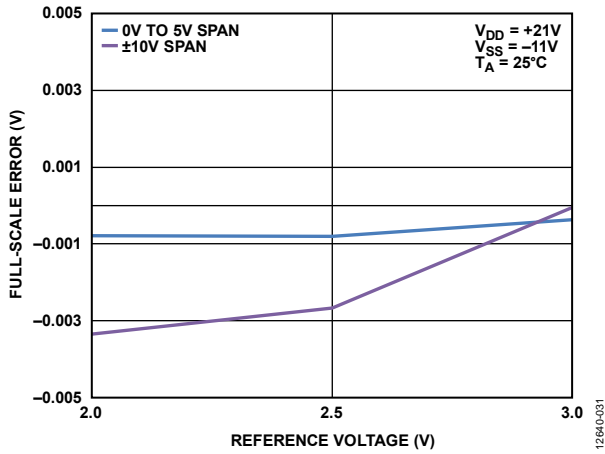
Figure 30. Full-Scale Error vs. Reference Voltage
