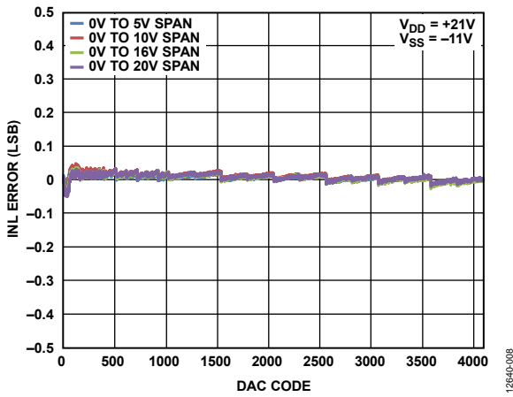
Figure 7. AD5721 INL Error vs. DAC Code, Unipolar Output
