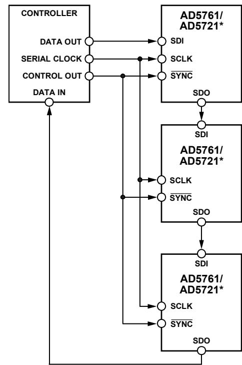
Figure 64. Daisy-Chain Block Diagram
