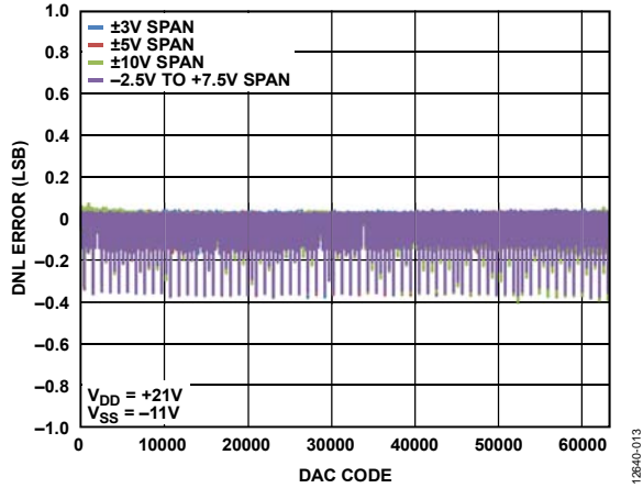
Figure 12. AD5761 DNL Error vs. DAC Code, Bipolar Output
