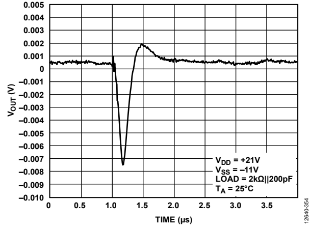
Figure 46. Digital-to-Analog Glitch Energy, 0 V to 5 V Range
