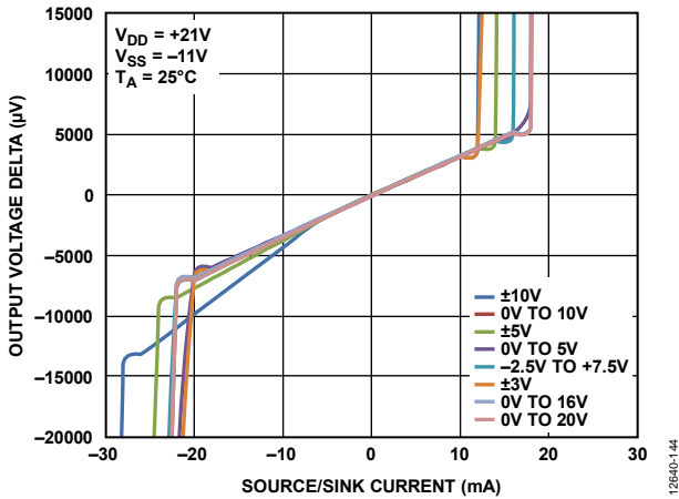
Figure 37. Source and Sink Capability of Output Amplifier with Negative Full Scale Loaded
