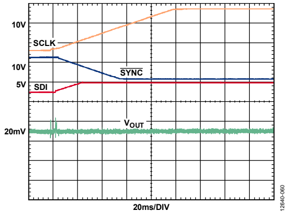
Figure 48. Power-Up Glitch
