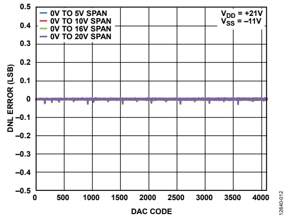
Figure 11. AD5721 DNL Error vs. DAC Code, Unipolar Output
