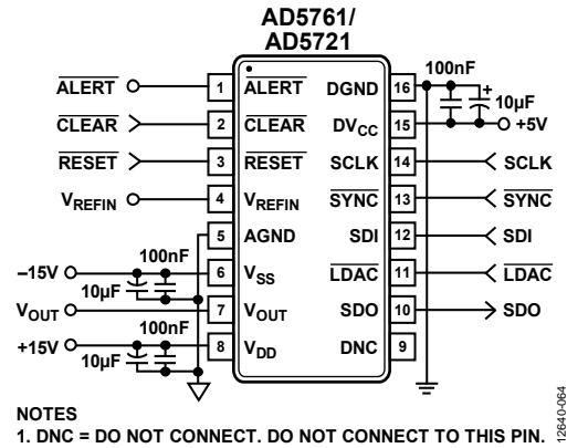
Figure 65. Typical Operating Circuit
