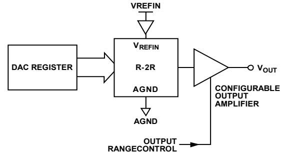
Figure 62. DAC Architecture
