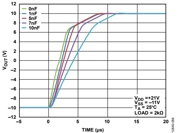
Figure 44. Settling Time vs. Capacitive Load, ±10 V Range
