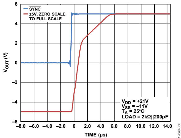
Figure 38. Full-Scale Settling Time (Rising Voltage Step), ±5 V Range
