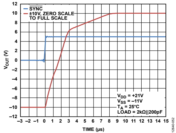
Figure 40. Full-Scale Settling Time (Rising Voltage Step), ±10 V Range
