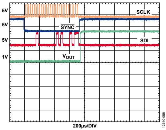
Figure 55. Output Range Change Glitch, 0 V to 5 V Range
