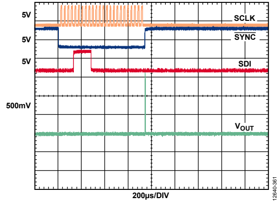
Figure 53. Software Full Reset Glitch from Midscale with Output Loaded, ±10V Range
