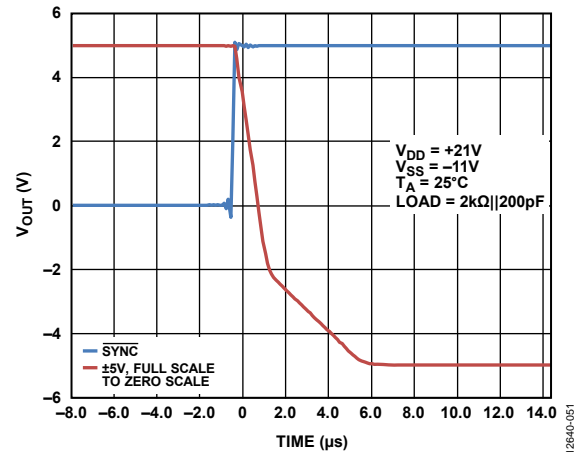
Figure 39. Full-Scale Settling Time (Falling Voltage Step), ±5 V Range
