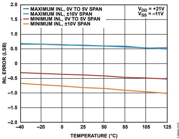
Figure 14. INL Error vs. Temperature
