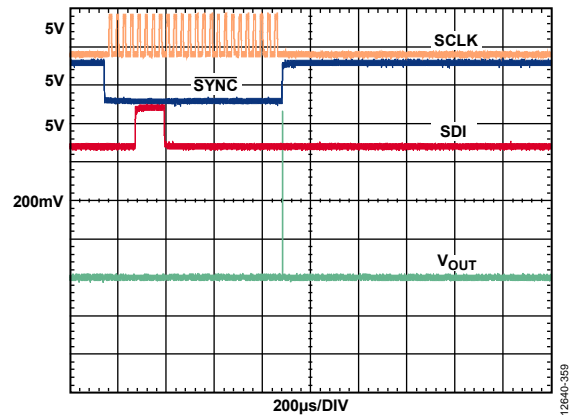
Figure 51. Software Full Reset Glitch from Zero Scale with Output Loaded, 0V to 5V Range
