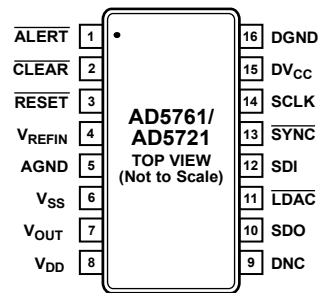
Figure 5. Pin Configuration
