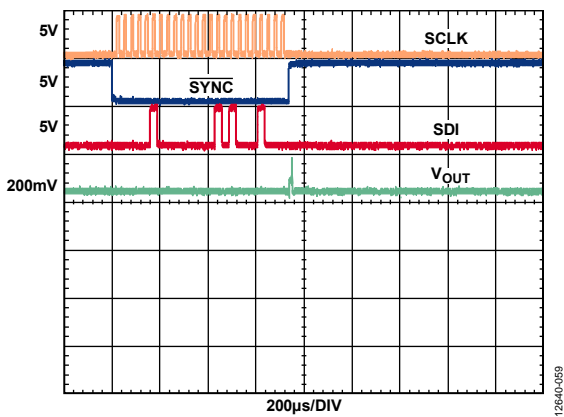
Figure 56. Output Range Change Glitch, \pm 10 V Range
