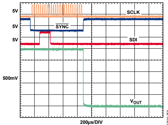
Figure 50. Software Full Reset Glitch from Midscale with Output Loaded, 0V to 5V Range
