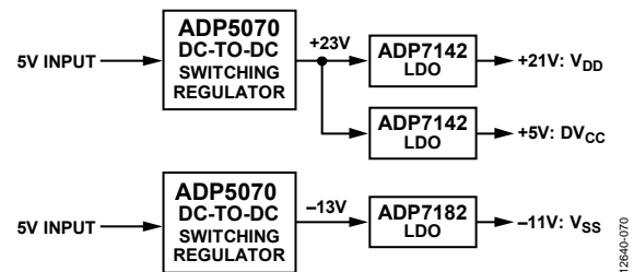
Figure 66. Postregulation by ADP7142 and ADP7182
