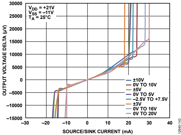
Figure 36. Source and Sink Capability of Output Amplifier with Positive Full Scale Loaded
