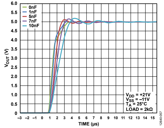
Figure 45. Settling Time vs. Capacitive Load, 0 V to 5 V Range
