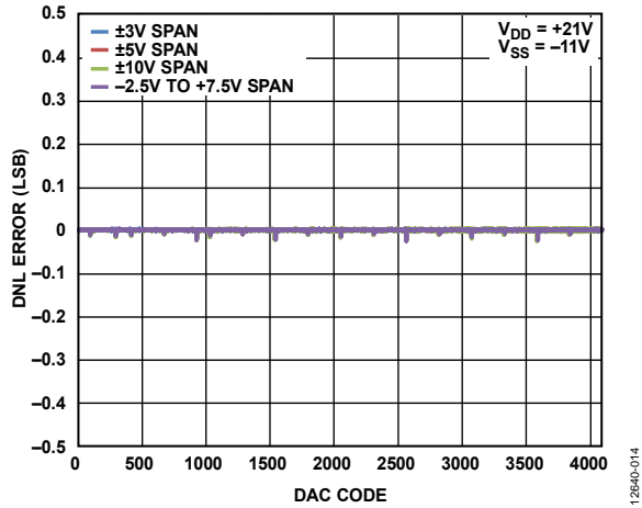
Figure 13. AD5721 DNL Error vs. DAC Code, Bipolar Output
