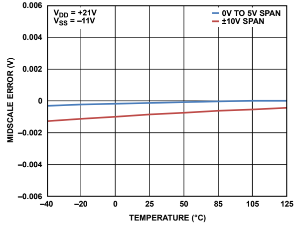
Figure 21. Midscale Error vs. Temperature
