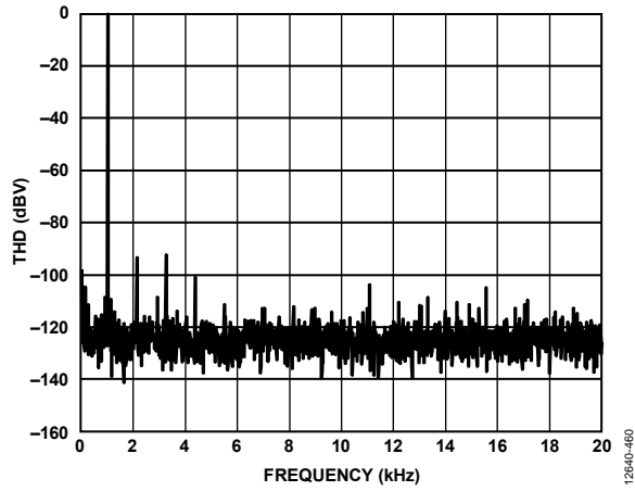
Figure 60. Total Harmonic Distortion at 1 kHz
