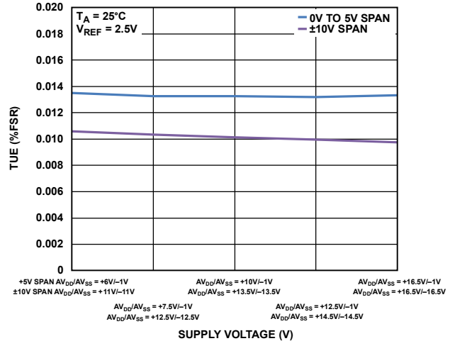
Figure 35. TUE vs. Supply Voltage
