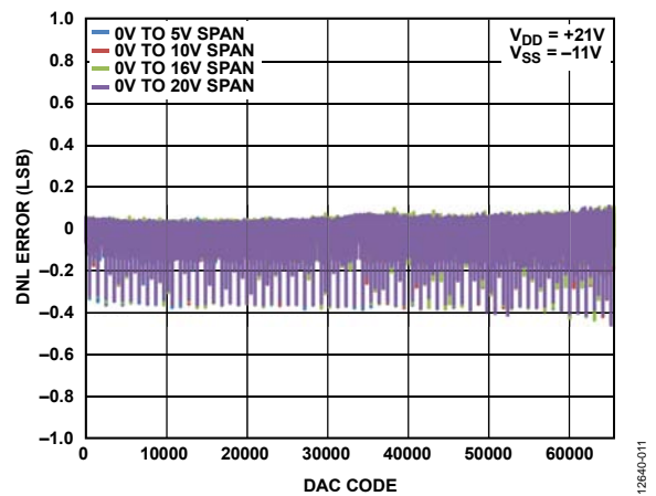
Figure 10. AD5761 DNL Error vs. DAC Code, Unipolar Output
