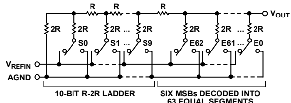
Figure 63. DAC Ladder Structure
