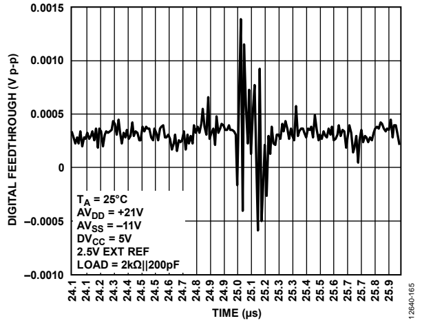
Figure 61. Digital Feedthrough
