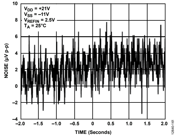
Figure 57. Peak-to-Peak Noise (Voltage Output Noise), 0.1 Hz to 10 Hz Bandwidth
