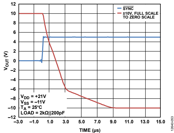
Figure 41. Full-Scale Settling Time (Falling Voltage Step), ±10 V Range
