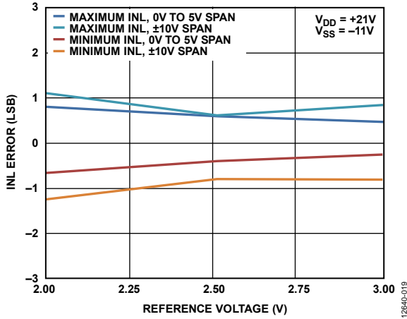
Figure 18. INL Error vs. Reference Voltage
