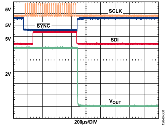
Figure 52. Software Full Reset Glitch from Full Scale with Output Loaded, ±10V Range
