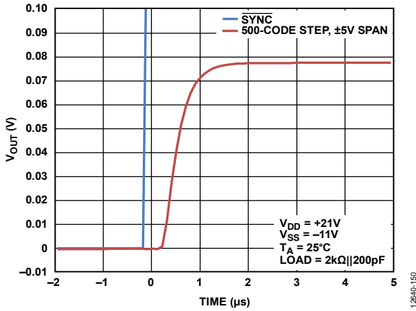
Figure 42. 500-Code Step Settling Time, ±5 V Range
