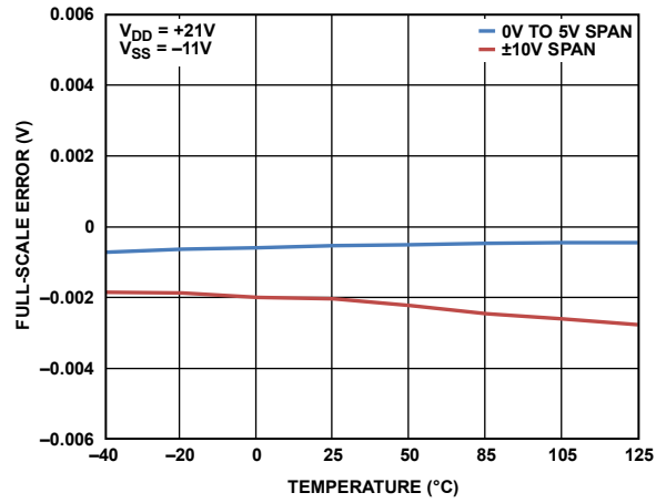
Figure 22. Full-Scale Error vs. Temperature
